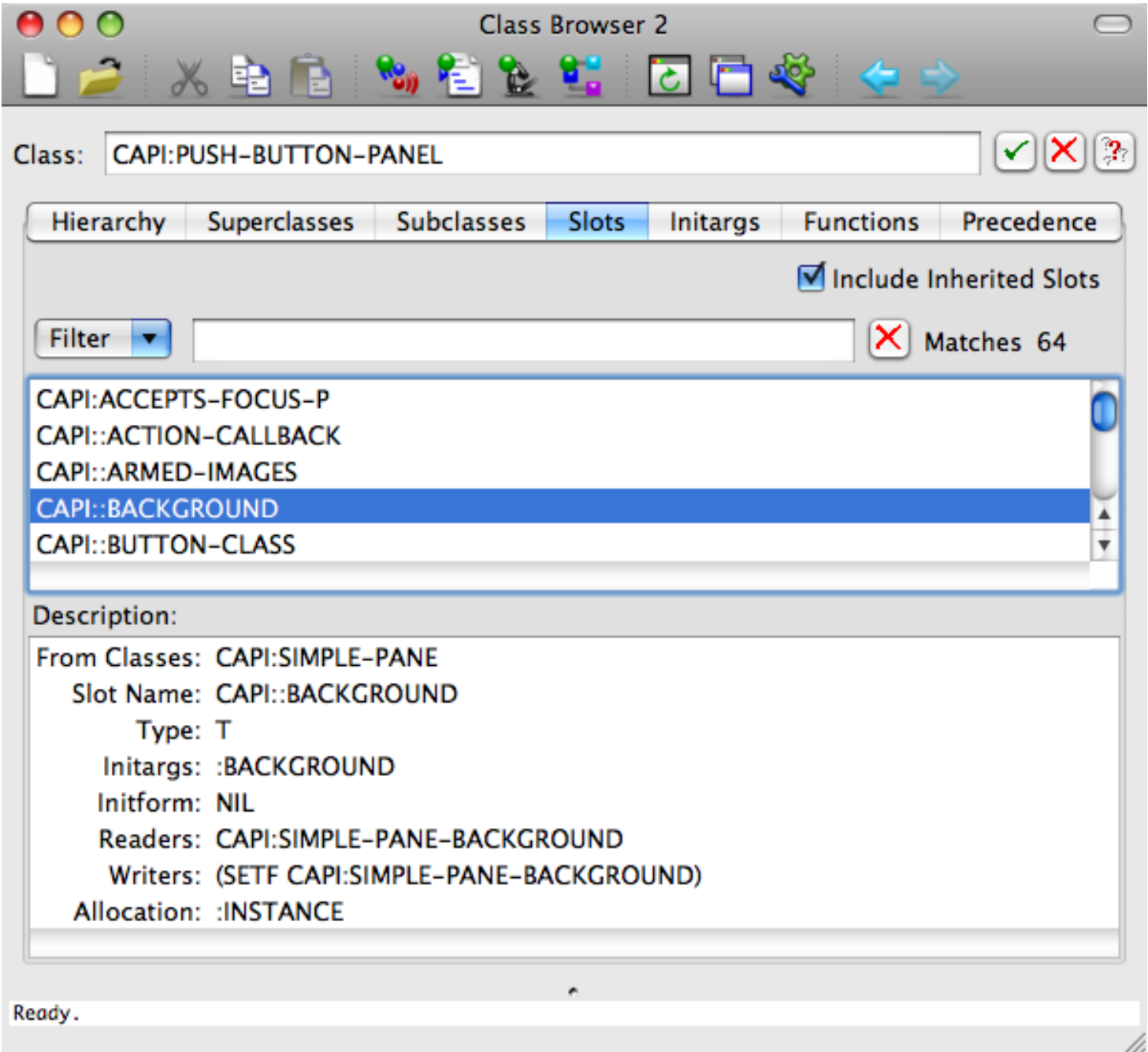
Examining slots in the Class Browser
