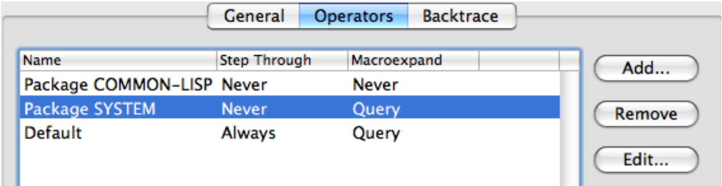
Stepper Preferences
