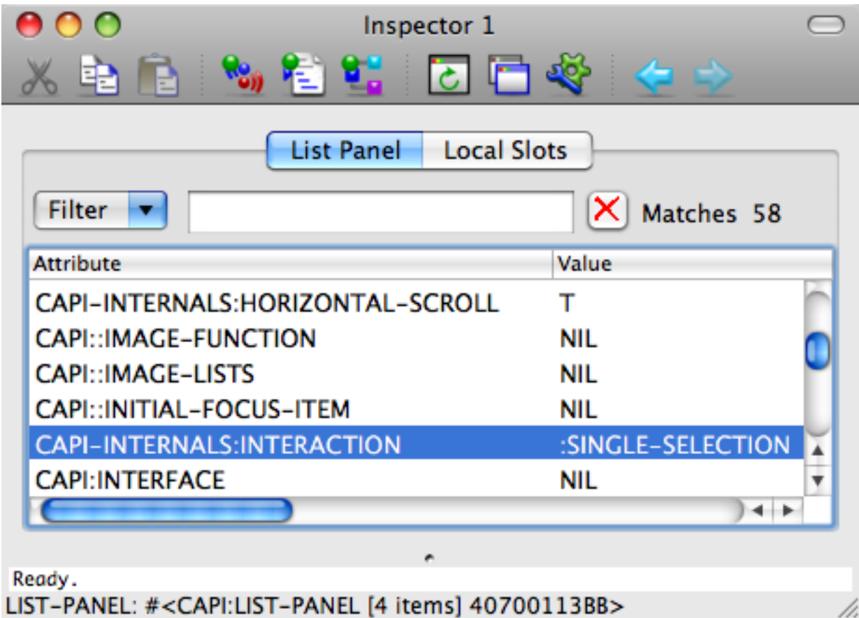
Inspector
