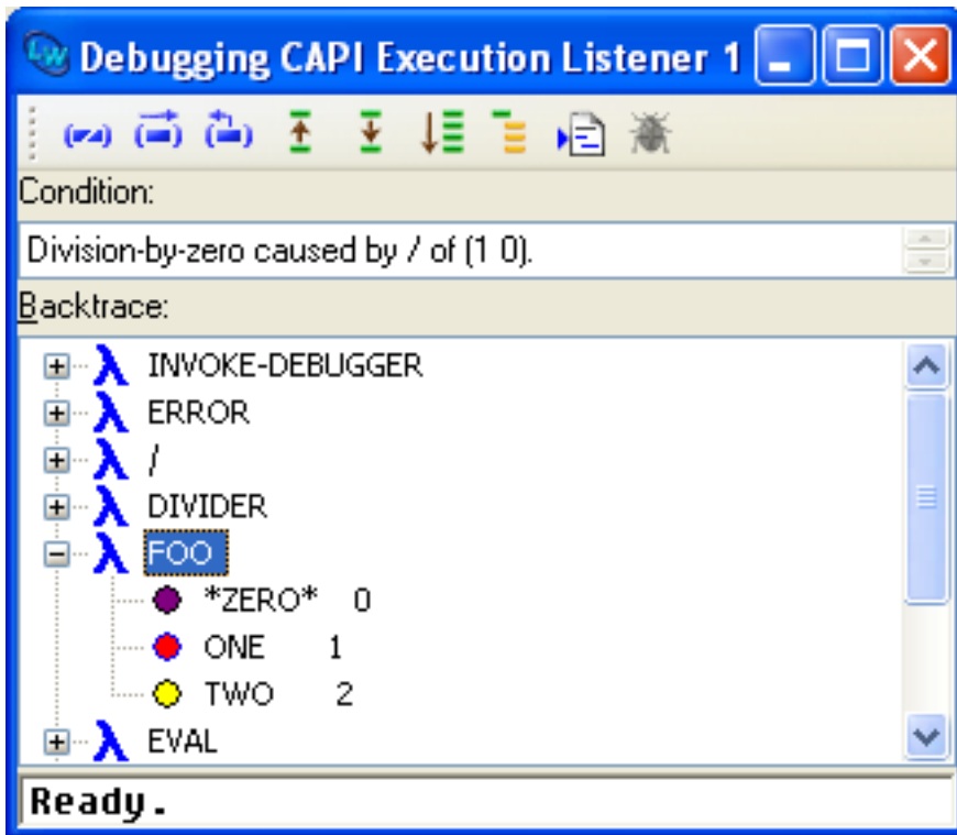
Variables in the Debugger tree view
