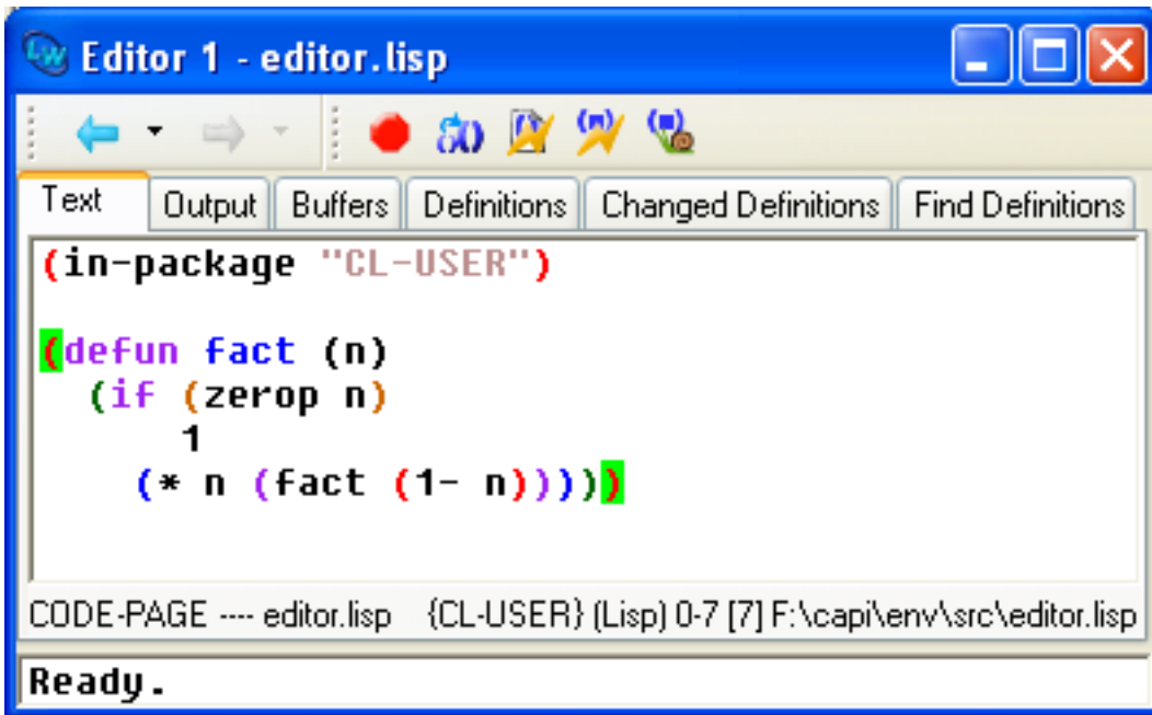
Text view in the Editor
