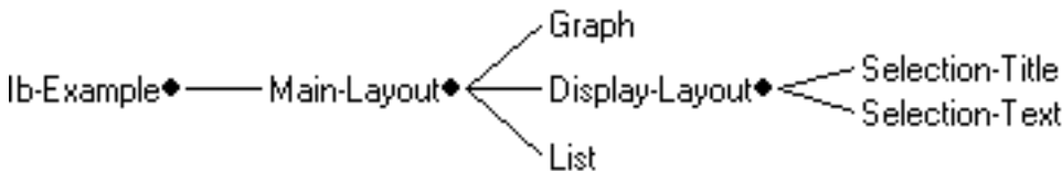
Layout hierarchy with names specified
