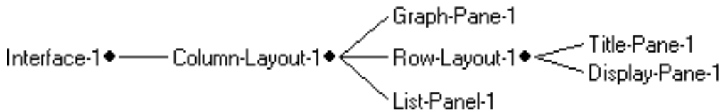
Layout hierarchy of the example interface
