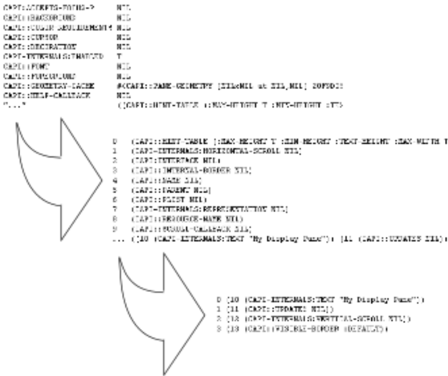
Displaying an object with more items than can be displayed
