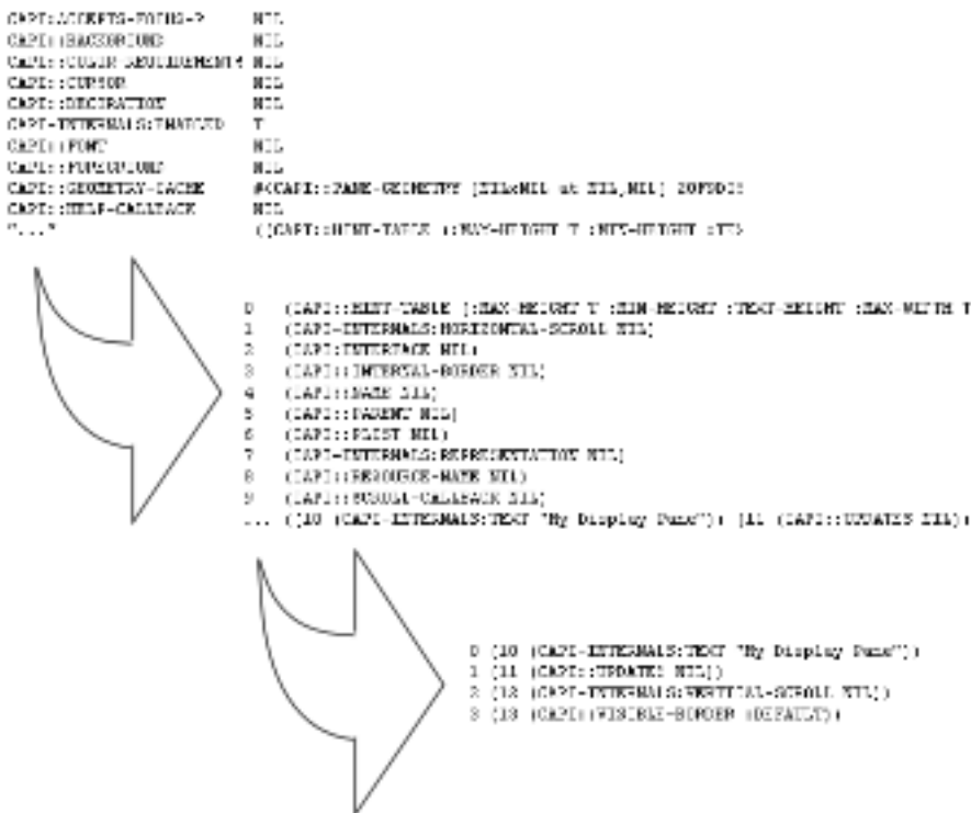
Displaying an object with more items than can be displayed
