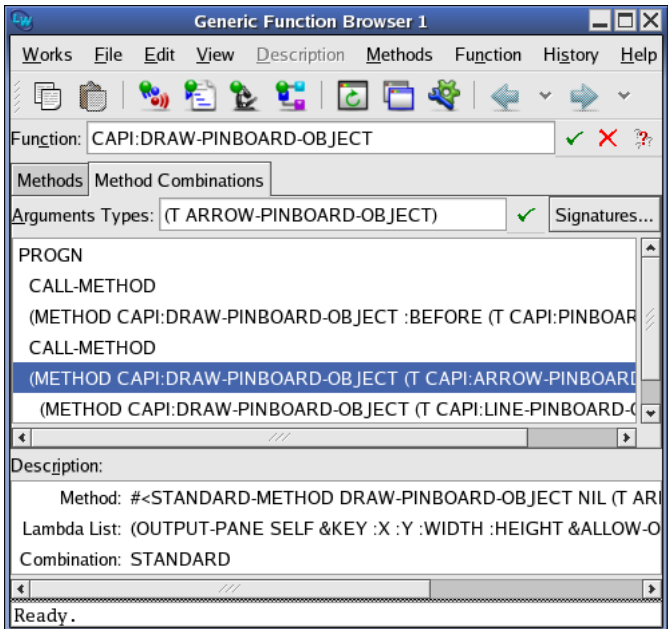
Generic function browser displaying method combinations
