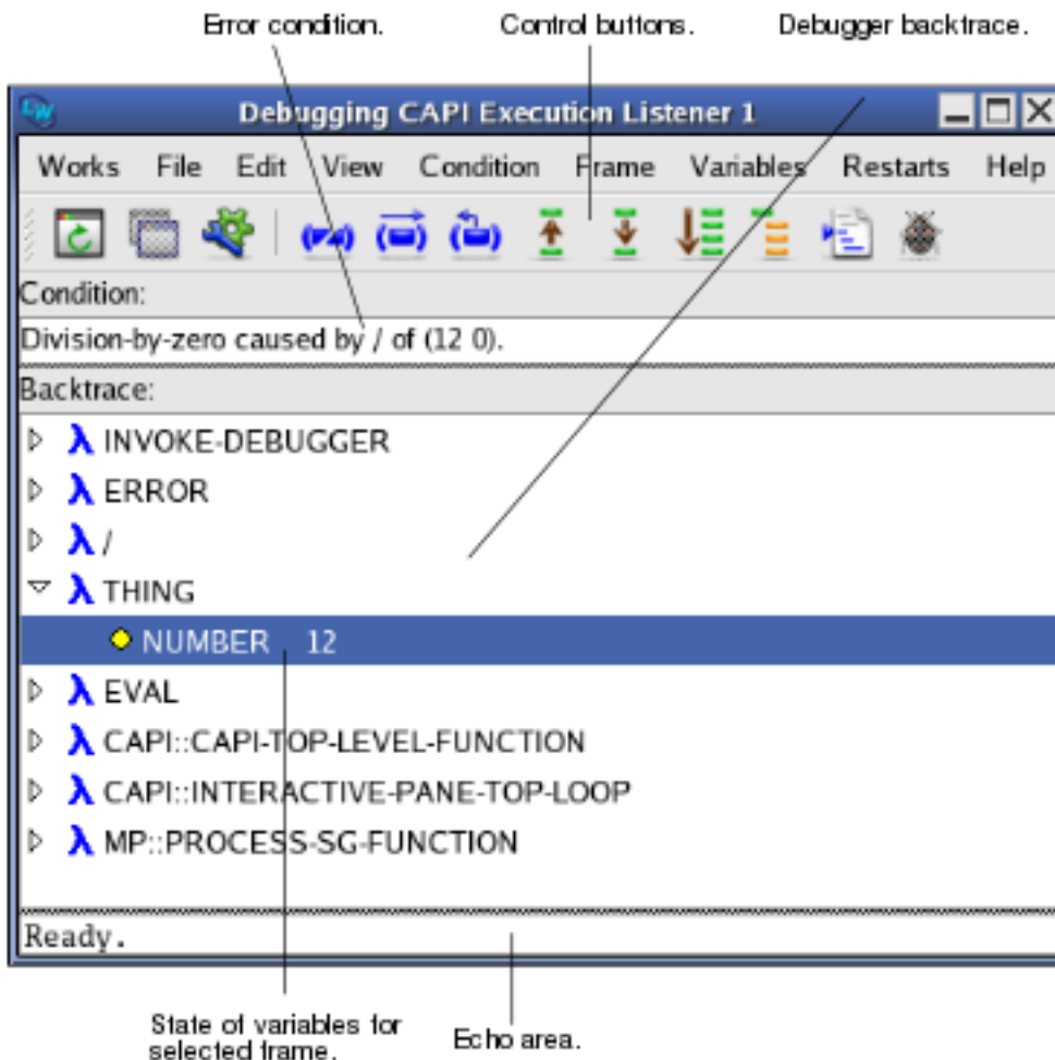
Debugger tool
