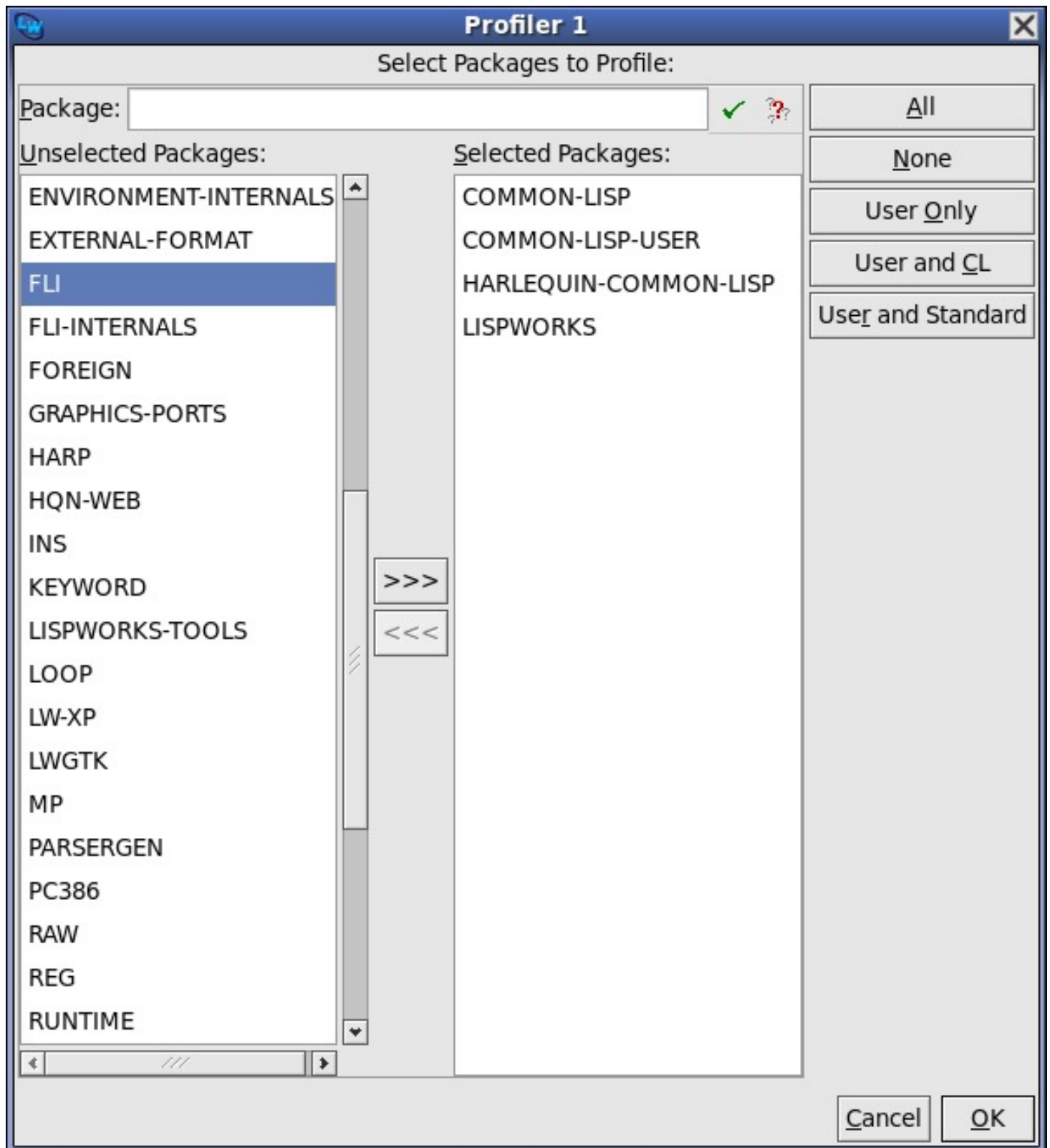
Select Packages to Profile dialog
