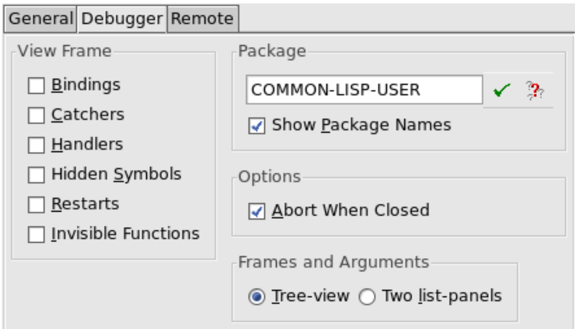
Debugger Preferences
