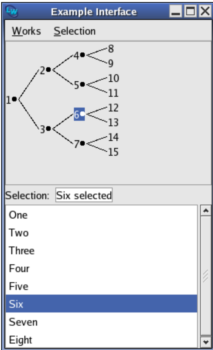
Example interface
